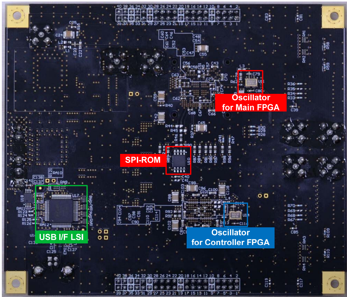
Figure 3 : SAKURA-G Board Functions (Bottom View)
