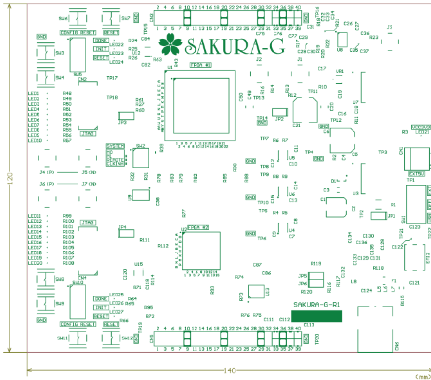
Figure 41 : Top Silk
